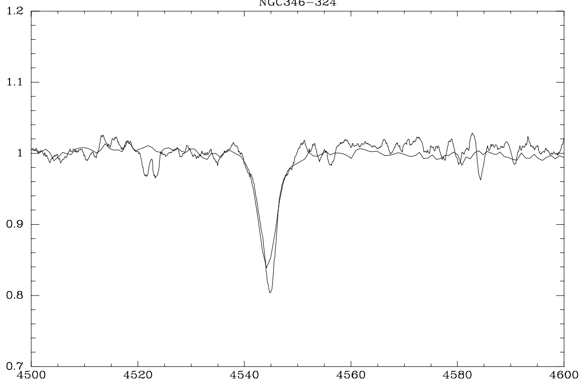
NGC346-324
