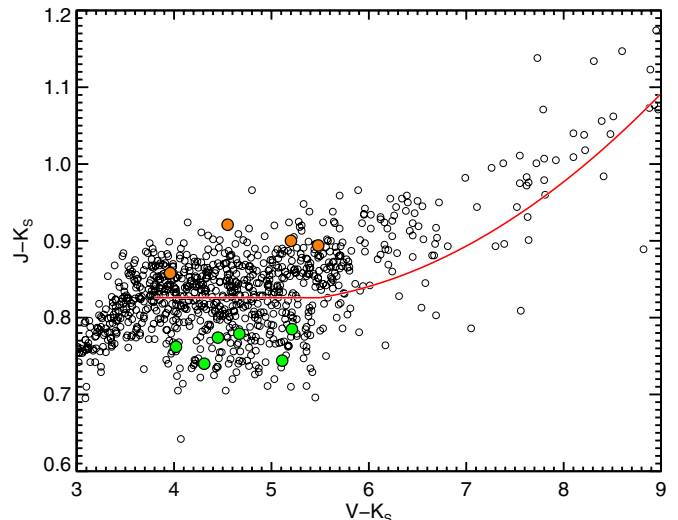
Figure 8. Color-color diagram for low-mass stars in the solar neighborhood. The “main sequence” is approximated by a constant for V - K < 5.5 , and a polynomial for redder values (solid line). Metal-rich M dwarfs known to have [\text{Fe}/\text{H}] > +0.25 as based on their FGK dwarf companions are highlighted above the main sequence (orange circles). Metal-poor stars with [\text{Fe}/\text{H}] < -0.25 are shown below the main sequence (green circles), indicating a relationship between metallicity and the distance a star lies away from the main sequence.
